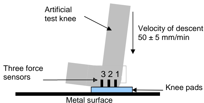
Figure 1: diagrammatic view of the bench for measuring the force distribution.
